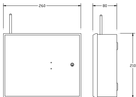
EDA-M300 Radio Repeater Panel
